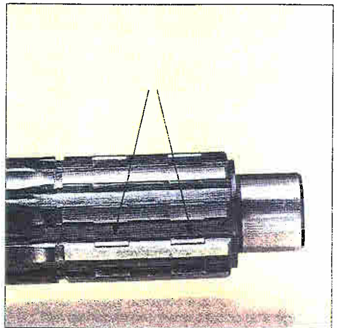
Figure 19—Worn shaft gearlocks can lead to gear jumping.
