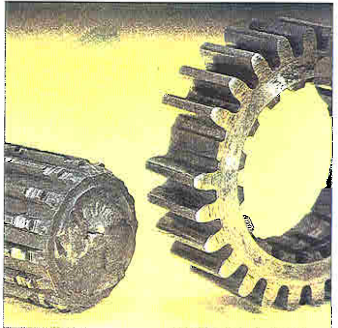
A broken shaft and missing gear teeth indicate shockload.
